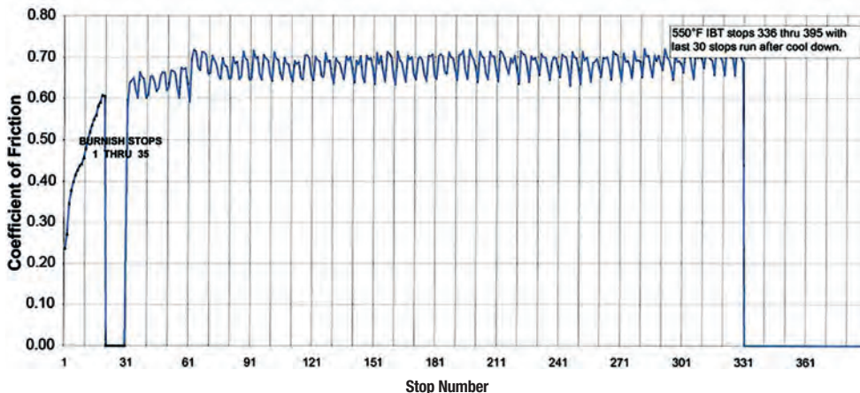
Dyno Graph
