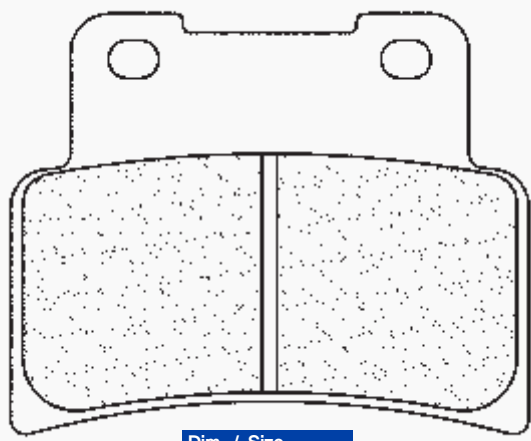
Dim. / Size 68.5 mm 55.5 mm 9 mm
